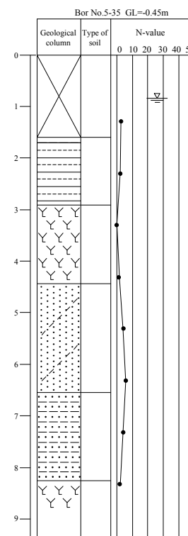
Figure 6. Geological conditions at vicinity of investigation ground measured by existing boring test
