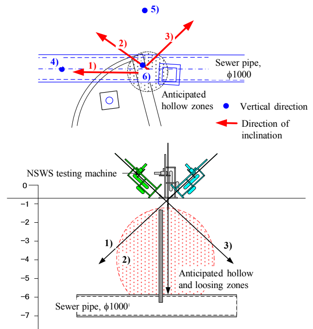
Figure 7. Outline of implementation plan for in-situ ground surveying with NSWS testing machine
