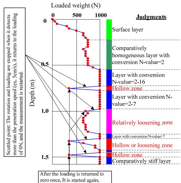
Figure 5. An example of result and interpretation on measurement with NSWS testing machine
