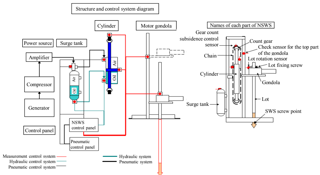
Figure 2. NSWS structure and applied load condition
