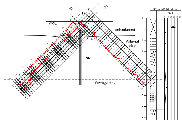
Figure 8. An example of testing result by NSWS testing machine in test hole 1)-3)
